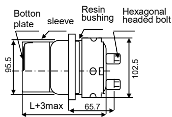
Method to mount resin bushing( \phi 76 )
