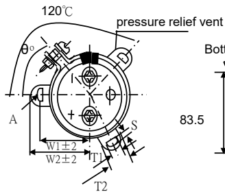
Method to mount resin bushing
